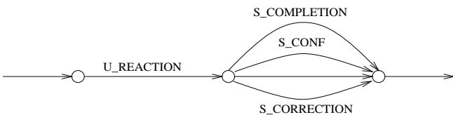
Figure 3: The REACTION/ subnet (cf. section 4).
