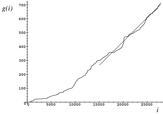
Figure 1: Estimation of the current OOV rate for the EVAR-system.
