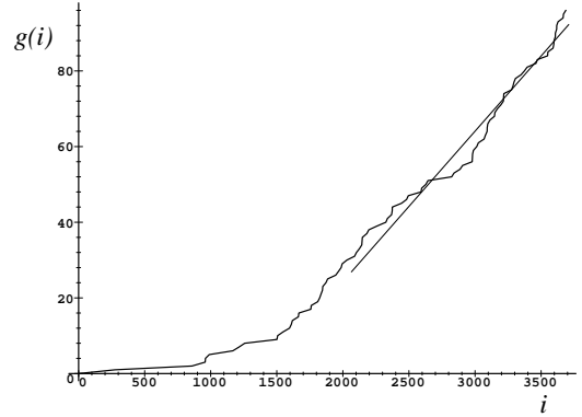
Figure 2: Estimation of the current OOV word probability for word category CITY.
