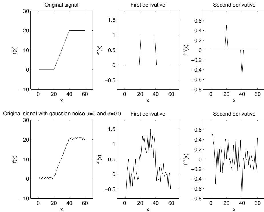
Figure 1: First row: original signal with clear distinguishable first and second derivative. Second row: signal with additive gaussian noise ( \mu = 0, \sigma = 0.9 ), first and second derivative respectively.
