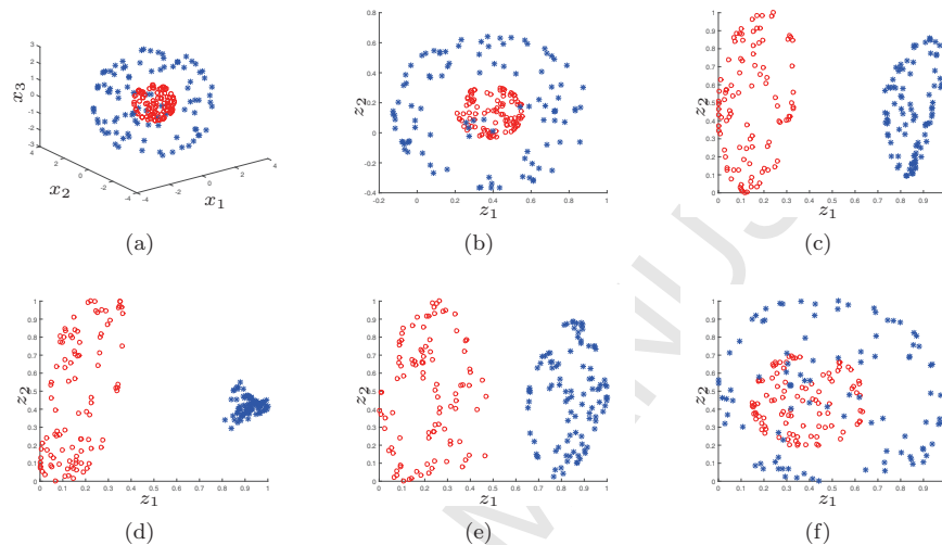
Figure 1: (a) Data points of one class from the unit sphere and are marked by red circles. The other data points, shown by blue stars, come from a sphere with radius 3. (b) This dataset is not linearly separable and thus linear PCA is not helpful for distinguishing the two classes. Instead, kernel PCA is needed and if the parameter is suitably chosen, the reduced data can be correctly classified by a linear classifier. (c) the RBF kernel with \sigma = 0.05 ; (d) the TL1 kernel with \rho = 0.1n ; (e) the TL1 kernel with \rho = 0.2n ; (f) the TL1 kernel with \rho = 0.5n , which is similar to linear PCA.
