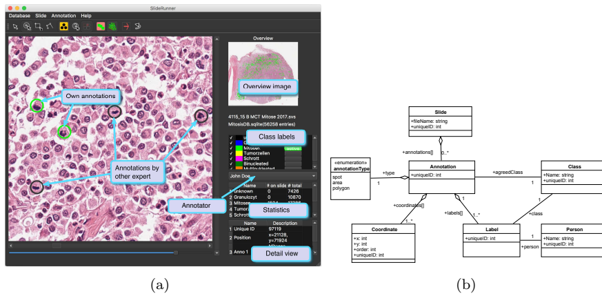
Figure 1: a) GUI overview in blinded mode. In this mode, annotations by other experts are only visible as unknown classes (in black). b) UML diagram of database structure. Every annotation may contain multiple labels from different persons and multiple coordinates.
