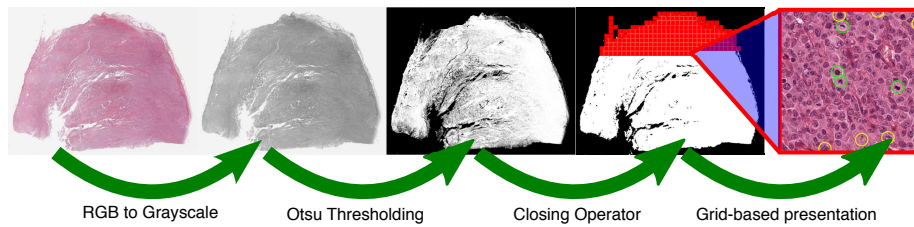
Figure 2: Algorithmic toolchain for guided screening. Grid-based segments are presented from left to right, top to bottom.
